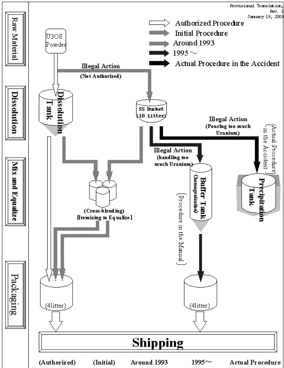
Figure 2 Change of Procedure to Produce Uranyl Nitrate at the Conversion Testing Building
